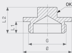
Čep - mesing Model 1751
