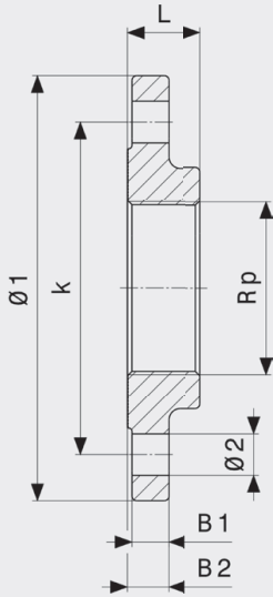
Sanpress XL-Prirubnica, PN 16 - bronca Model 2259.2XL
