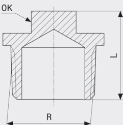
Čep - bronca Model 3290
