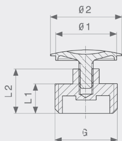
Čep - mesing Model 1752
