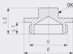
Čep - mesing Model 1751
