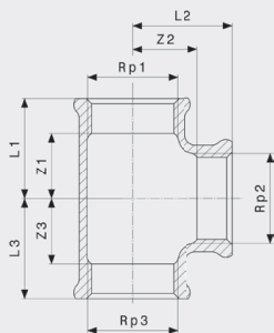
T-komad - bronca Model 3130
