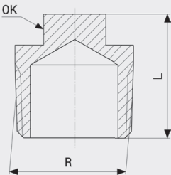
Čep - bronca Model 3291
