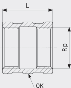
Spojnicica - bronca Model 3270
