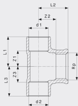
T-komad - bronca Model 94130G
