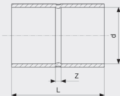
Spojnica - bakar Model 95270
