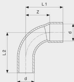
Koljeno 90° - bakar Model 95001A
