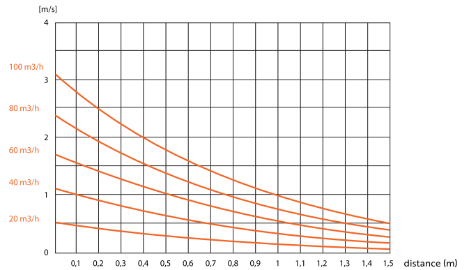
KVADRO 100/125 velocity, m/s
