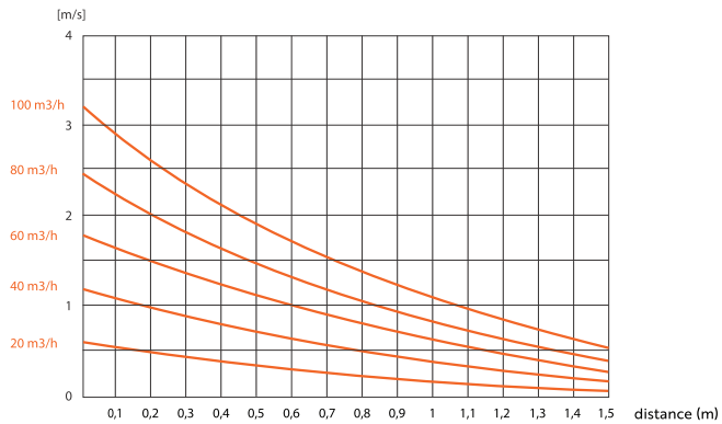
RONDO 100/125 velocity, m/s
