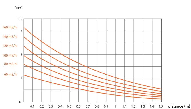
RONDO 150/160 velocity, m/s
