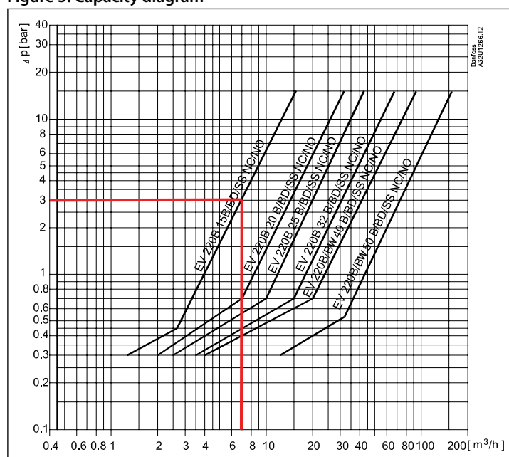
Figure 5: Capacity diagram
