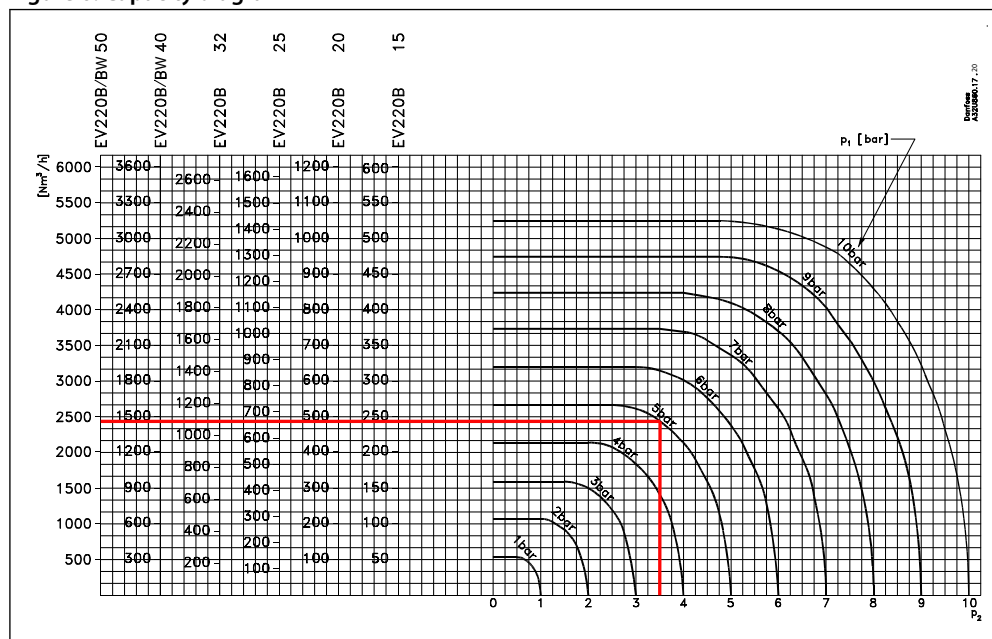
Figure 6: Capacity diagram
