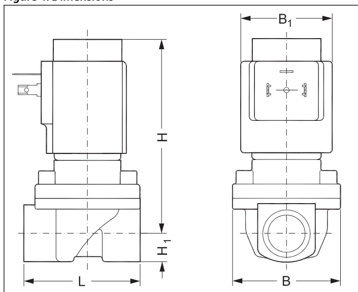
Figure 4: Dimensions
