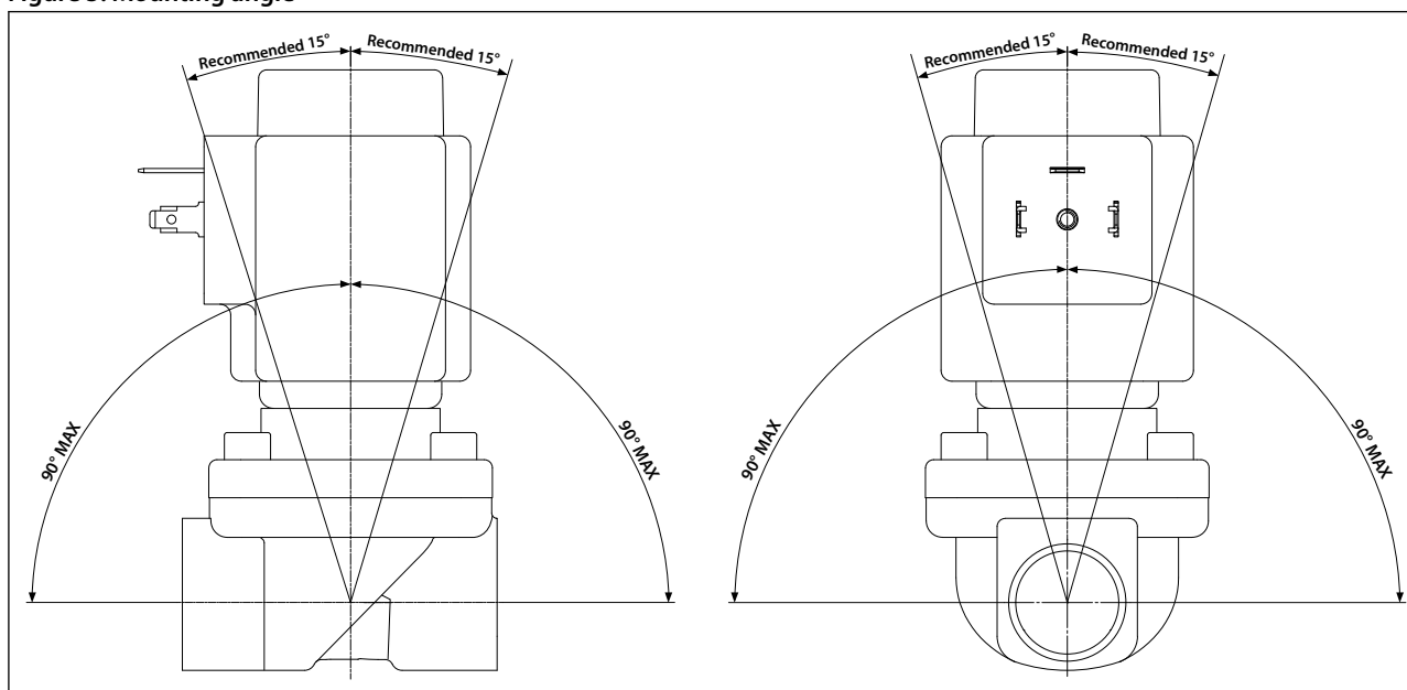
Figure 5: Mounting angle
