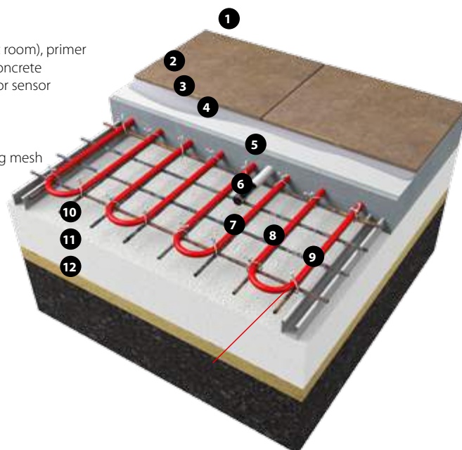
Fig. 5. Cable heating in concrete with cable fixed to reinforcement mesh by plastic cable ties.
