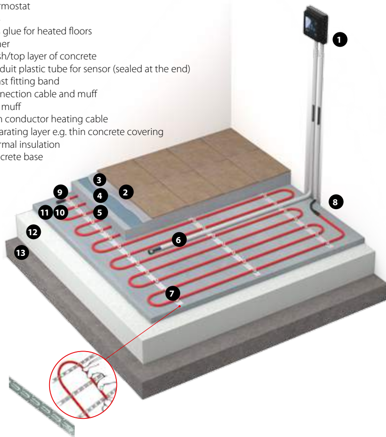
Fig. 4. Cable heating in concrete floor with cable fixed by ECfast fitting band.
