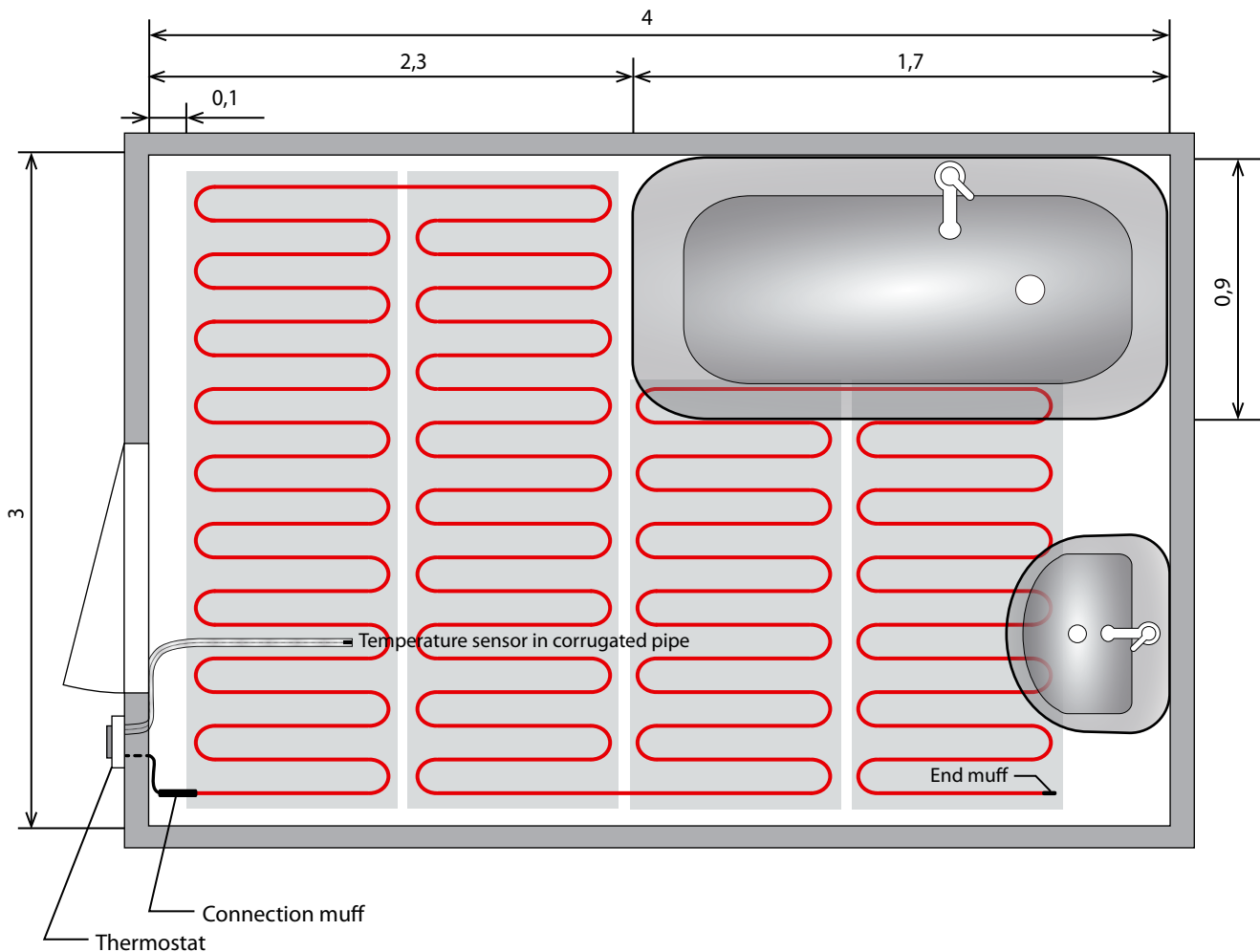
Fig. 1 – Example of heating mat installation in bathroom. All distances are in [m].
