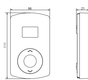
Fig. 2: Room Thermostats
