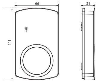
Fig. 4: CF-RU Repeater Unit
