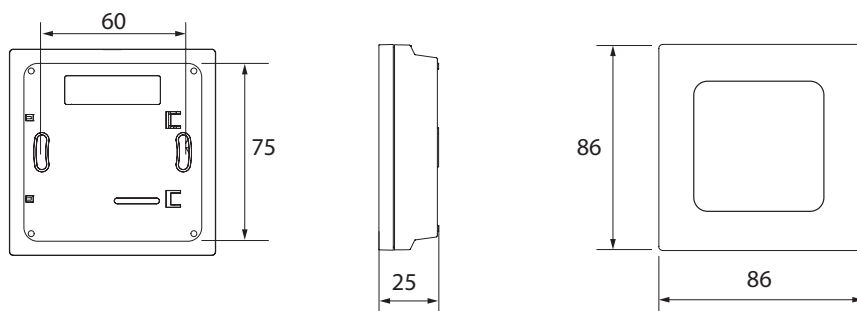
Danfoss Icon ™ 088U1015 Display
