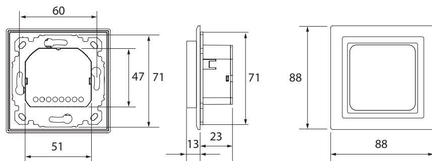
Danfoss Icon ™ 088U1012 Display (uklj. okvir Feller EDIZIOdue i adapter)
