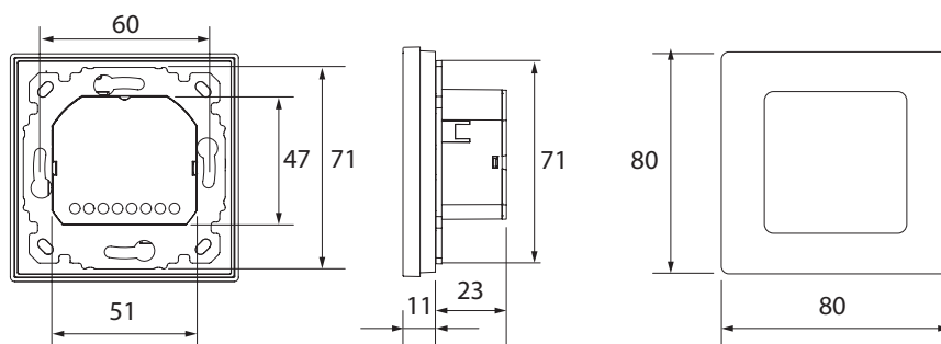
Danfoss Icon ™ 088U1010 Display
