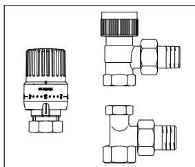
Abb.1 TRV9-Set, Eckform
