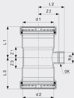
Prestabo XL-T-komad - nelegirani pocinčani čelik Model 1117.2XL
